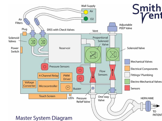
Figure 3: Rendering of Smith Vent design
