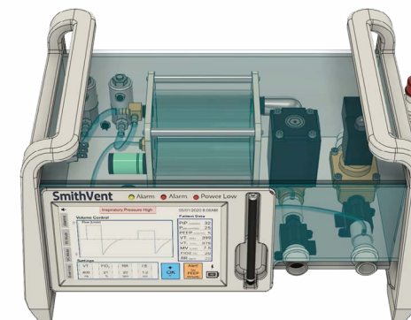
Figure 3: Rendering of Smith Vent design
